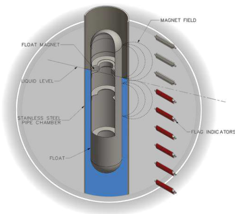
Aquarian 4000 Magnetic Level Indicator (MLI)
