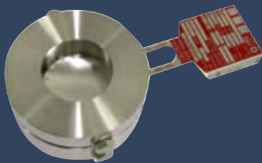
Rupture Disc holder and disc assembly
