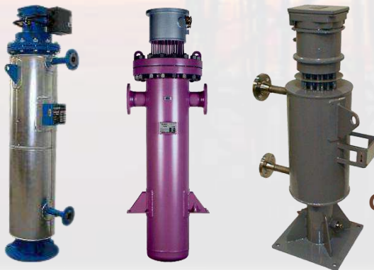
Ex- Immersion Heaters Fluid, Air, Gas and Compact Body
