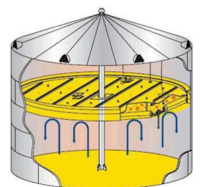
Vapor Prevention with Floating Roof
