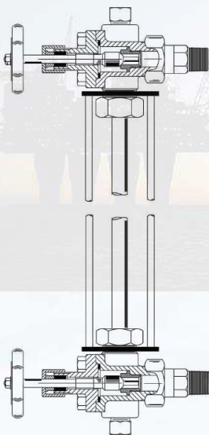
Tubular Liquid Level Gauge
