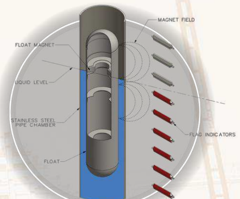
Aquarian 4000 Magnetic Level Indicator (MLI)
