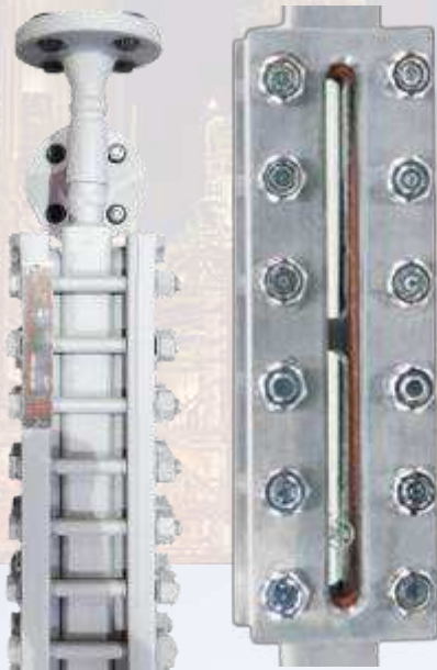
Transparent Liquid Level Gauge
