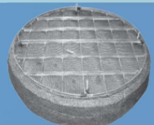
Demister Pad
