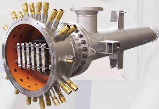
Process Heater
